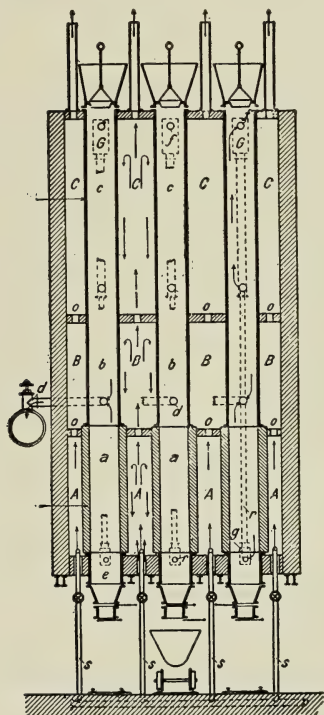
FIG. 82.—Retort for Distilling Impure Lignite.
